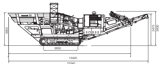
Side view IC 50
