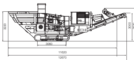
Side view IC 35
